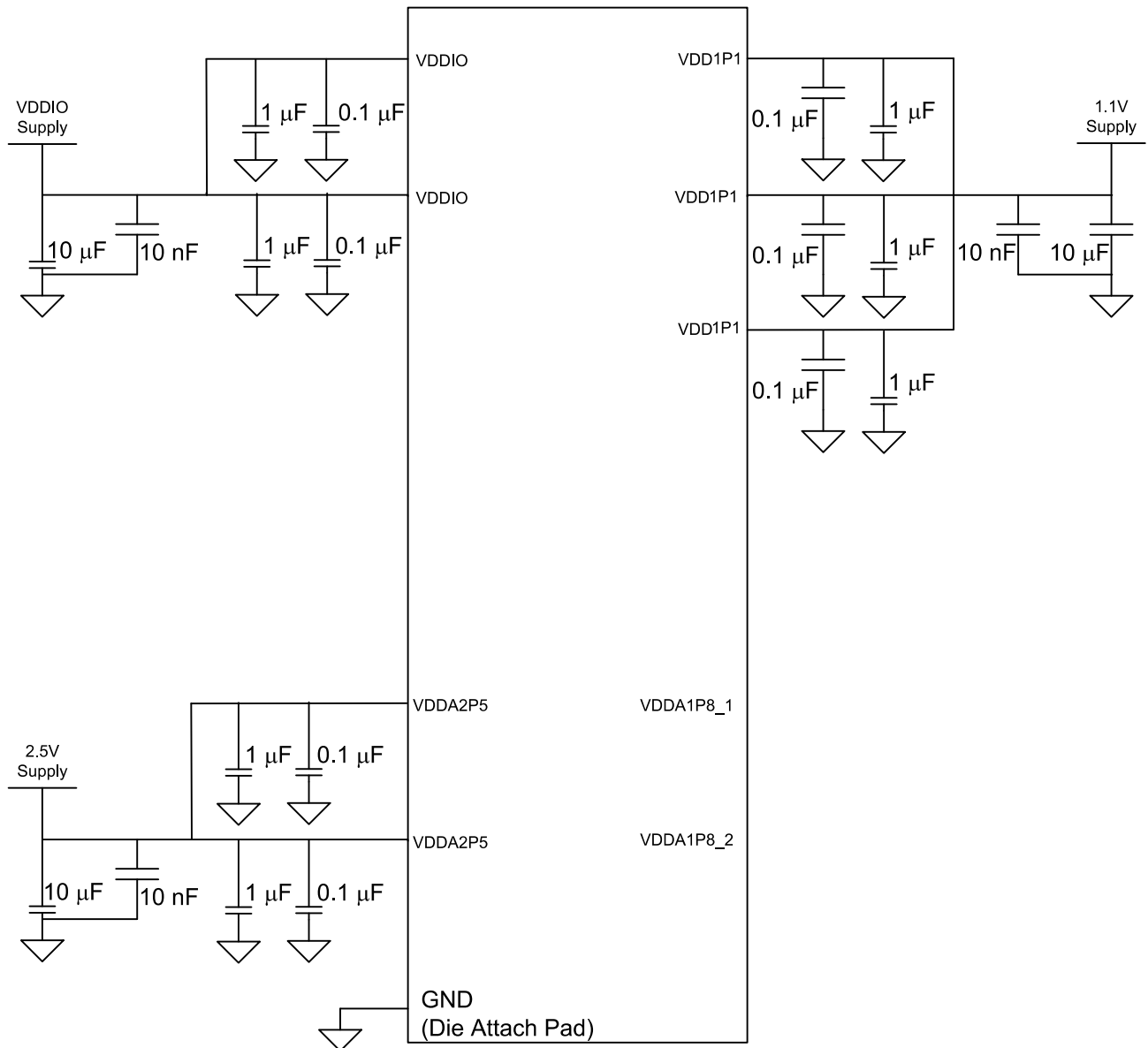
Figure 8-6. Two-Supply Configuration
