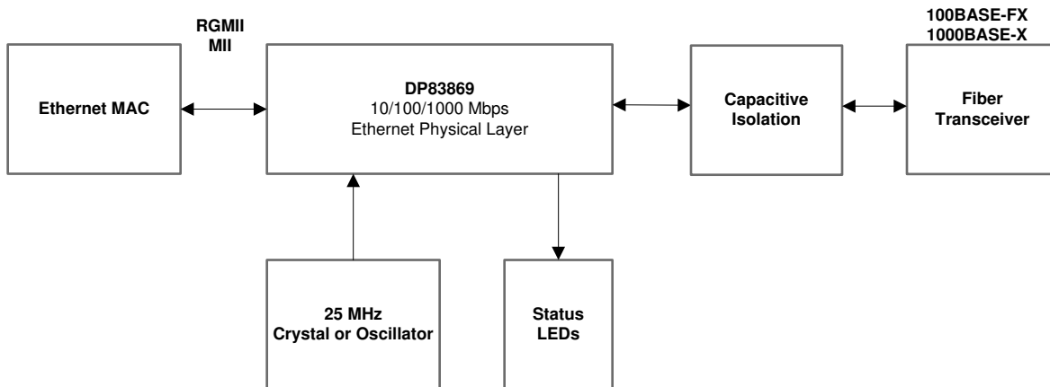
Figure 8-4. Typical Fiber Ethernet Application
