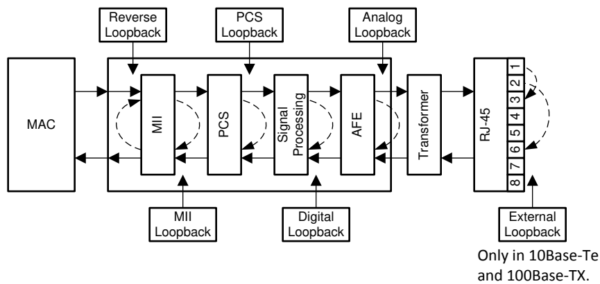
Figure 7-4. Loopbacks
