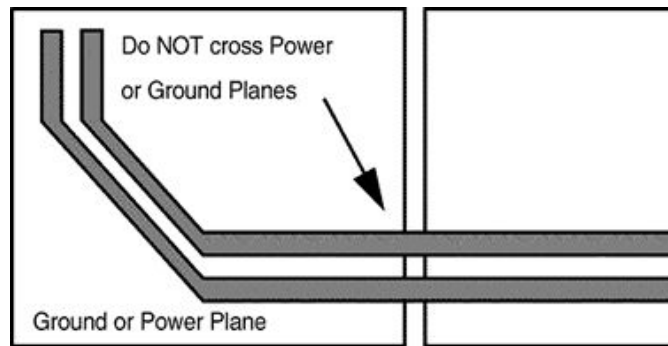
Figure 8-11. Differential Signal Pair-Plane Crossing
