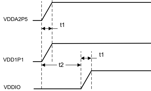
Figure 8-7. Two-Supply Sequence Diagram
