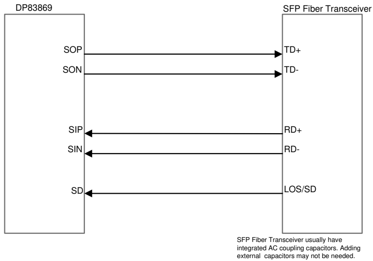
Figure 8-5. PHY to Fiber Transceiver Connections
