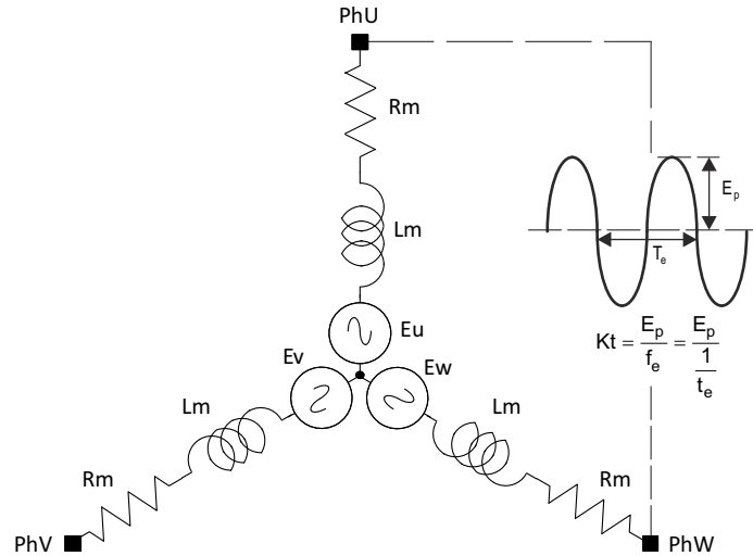
Figure 8-9. K_{t_{PH}} Definition
