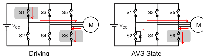
Figure 8-35. Inductive AVS
