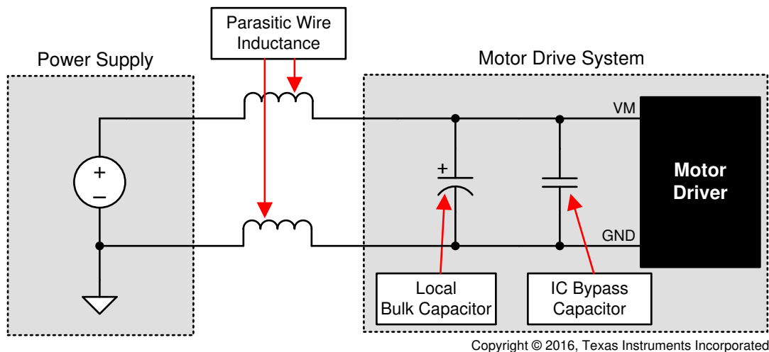
Figure 7-11. Example Setup of System With External Power Supply
