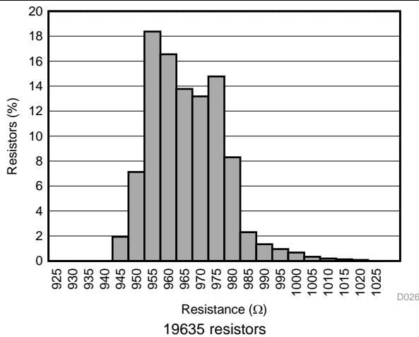
Figure 41. Resistor Absolute Value Histogram
