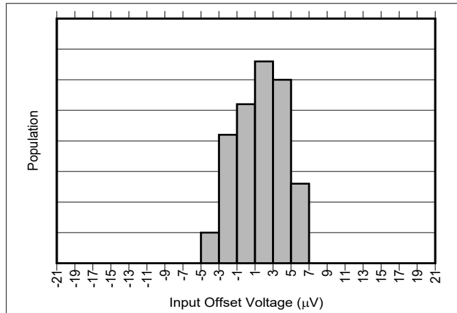
Figure 6-1. INA241A1-Q1 Input Offset Production Distribution
