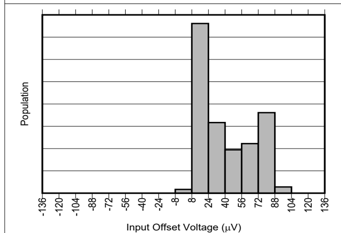
Figure 6-3. INA241A3-Q1 and INA241A4-Q1 Input Offset Production Distribution
