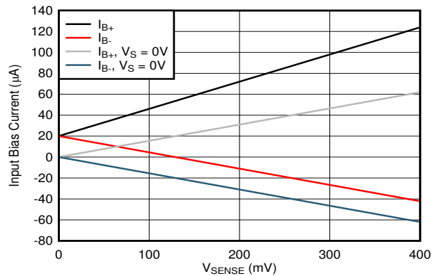
Figure 6-16. INA293x2, INA293x3 Input Bias Current vs V_{SENSE}
