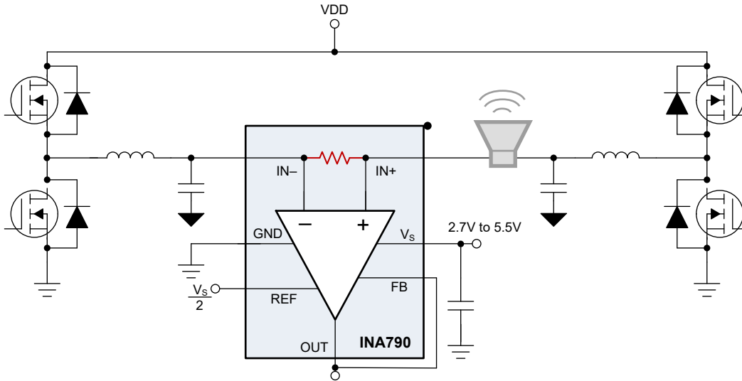
Figure 7-2. Current Sensing in a CLASS-D Subsystem
