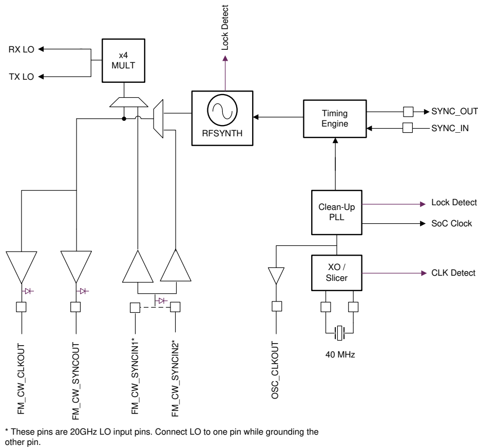
Figure 9-1. Clock Subsystem
