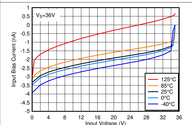
Figure 6-18. Input Bias Current vs. Input Voltage at 36V
