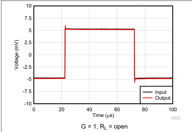
Figure 5-29. Small-Signal Step Response, G = 1
