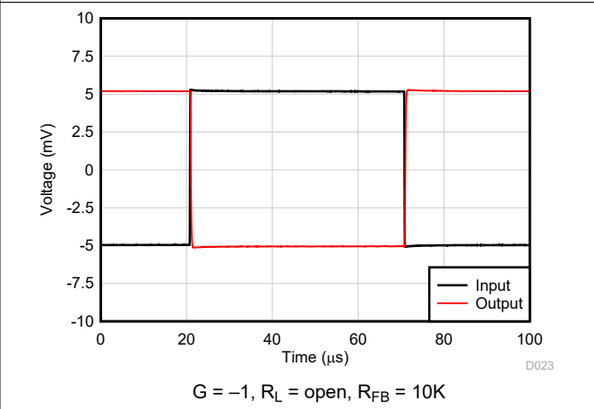
Figure 5-30. Small-Signal Step Response, G = -1
