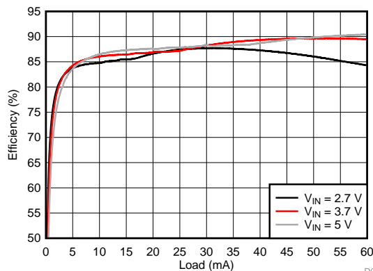
Backlight Efficiency, 2P8S
