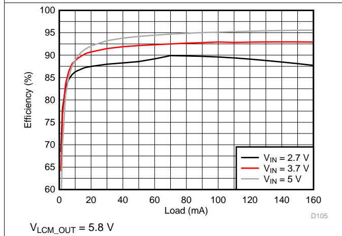
Figure 119. LCM Boost Efficiency
