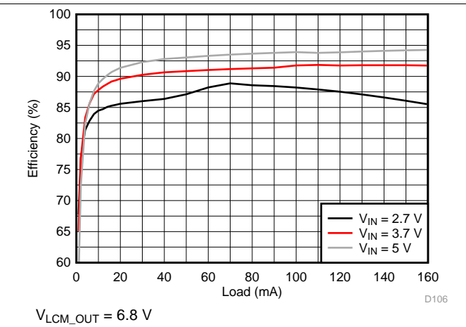
Figure 120. LCM Boost Efficiency
