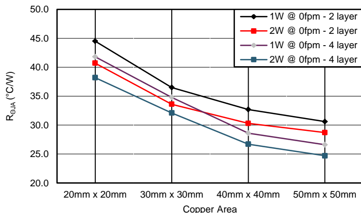
Figure 101. Measured R θJA vs PCB Copper Area on a 2-layer Board and a 4-layer Board
