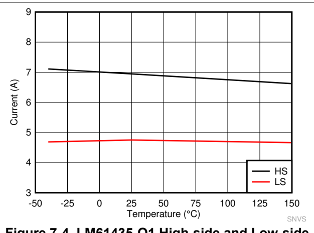
Figure 7-4. LM61435-Q1 High-side and Low-side Current Limits
