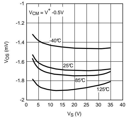
Figure 20. V_{OS} vs. V_S (Unit 1)
