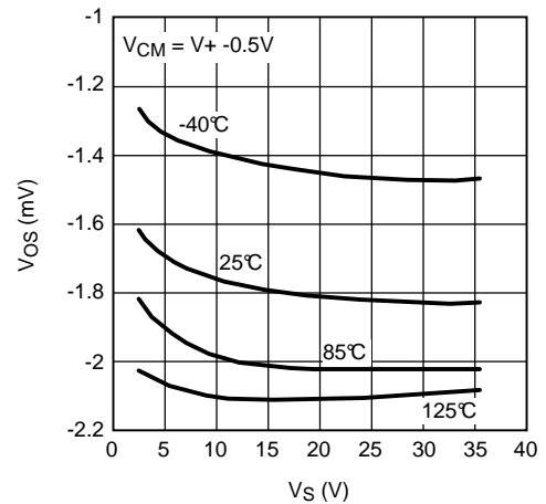
Figure 22. V_{OS} vs. V_S (Unit 3)
