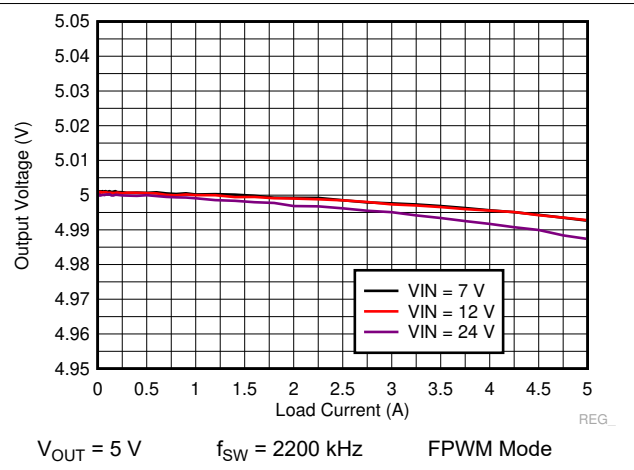
Figure 9-26. LM73605-Q1 Load and Line Regulation
