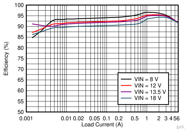
Figure 9-9. LM73605-Q1 Efficiency
