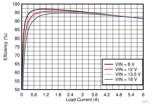
Figure 9-10. LM73605-Q1 Efficiency
