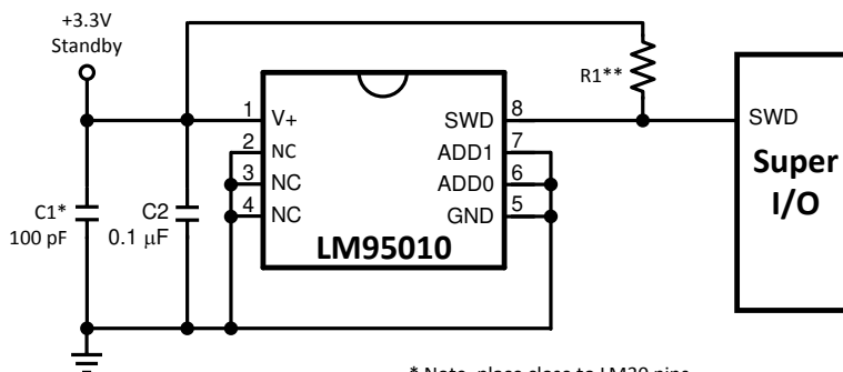
LM95010 connection to SensorPath master such as a Super I/O.
