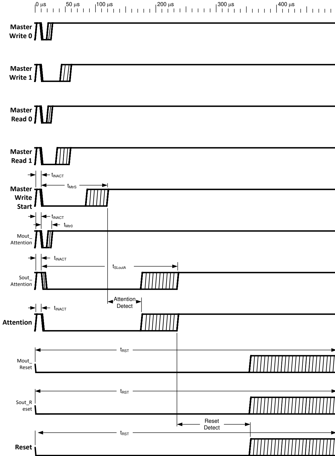
Figure 5-3. Timing for Attention Request and Reset
