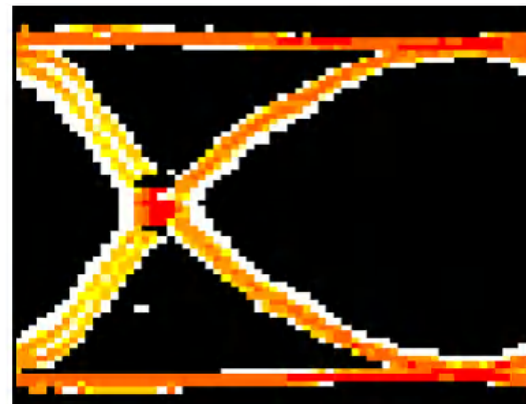
Figure 8-3. Internal Eye Monitor Hit Density Plot
