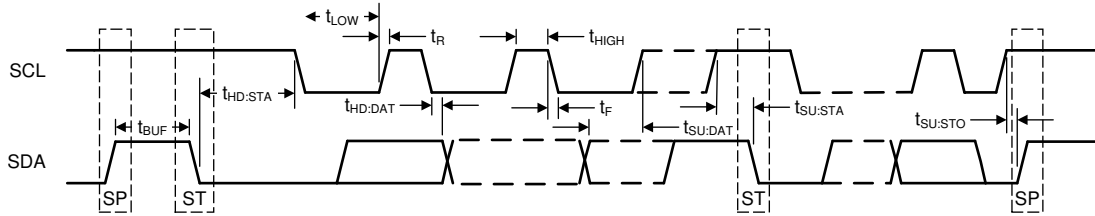
Figure 7-1. SMBus Timing Parameters
