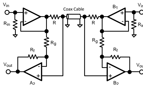
Figure 30. Full Duplex Transmit and Receive Using the LMH6628
