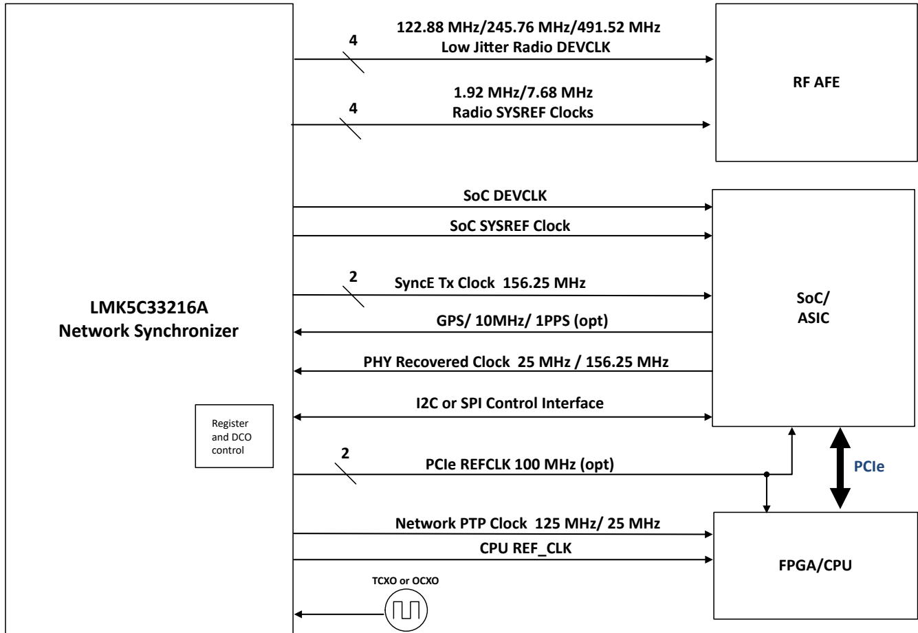
LMK5C33216A Typical System Block Diagram
