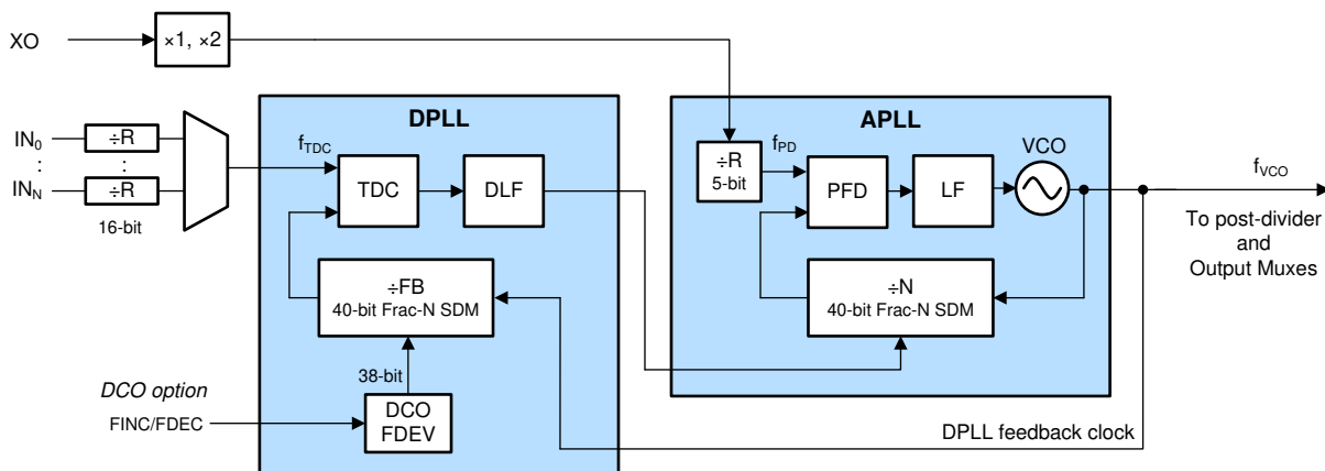
Figure 7-21. PLL Architecture
