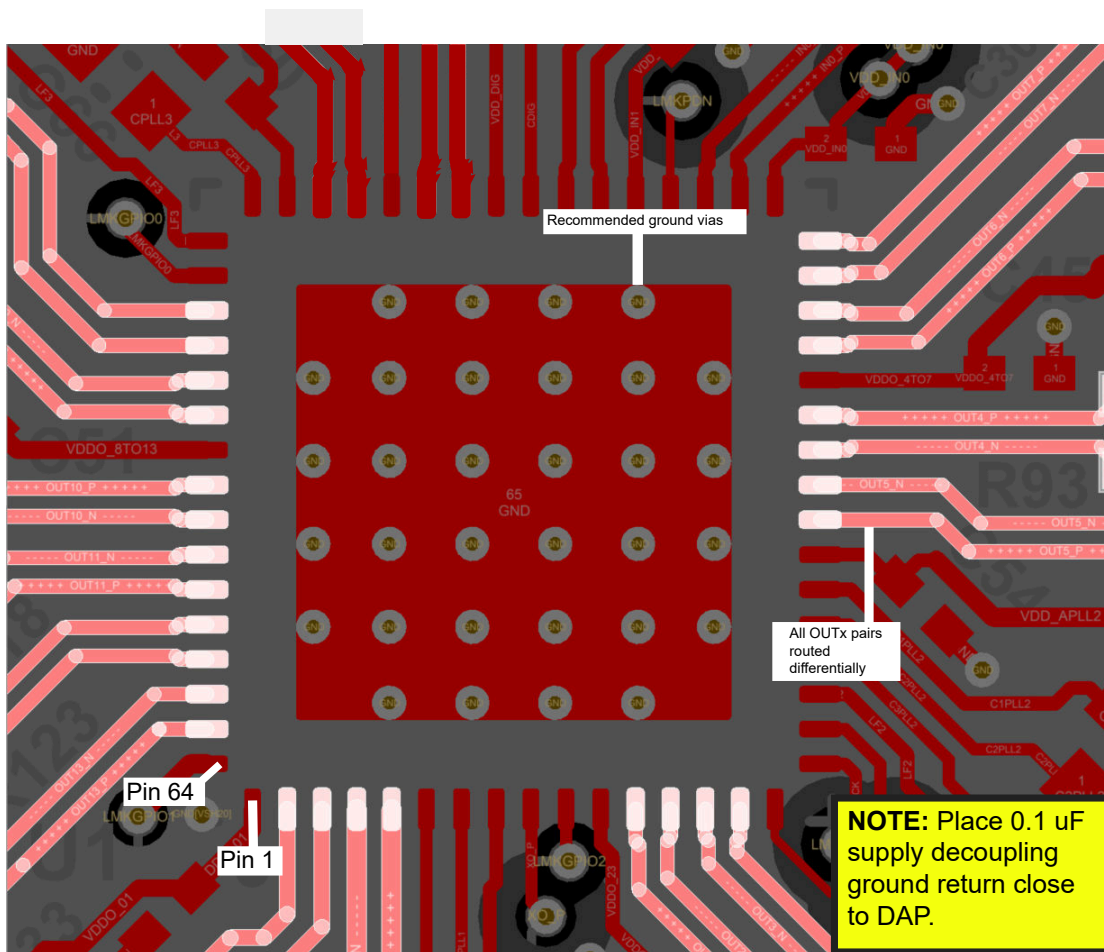
Figure 8-5. PCB Layout Example for LMK5C33216A, Top Layer
