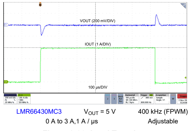
Figure 8-30. Load Transient
