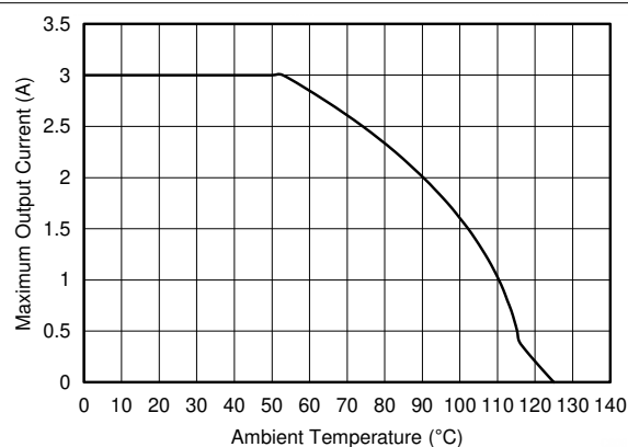
Figure 9-4. Maximum Output Current vs Ambient Temperature
