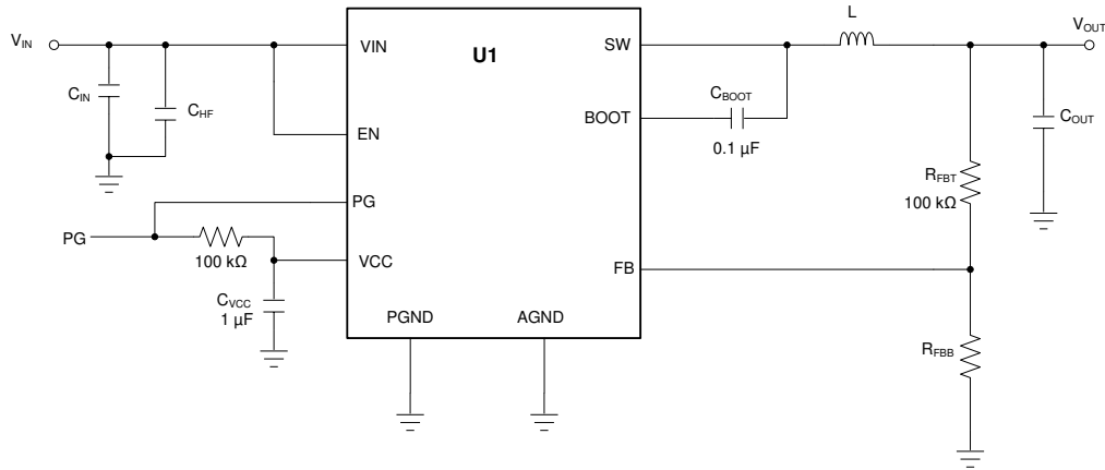
Figure 9-27. Circuit for Application Curves
