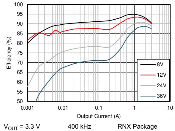
Figure 9-6. Efficiency
