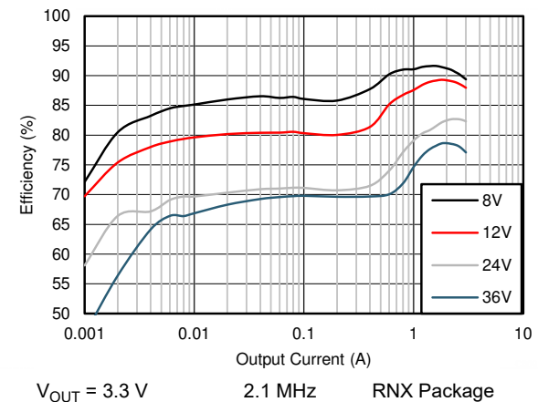
Figure 9-8. Efficiency
