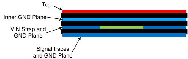
Figure 11-2. Example Layout for VQFN Package
