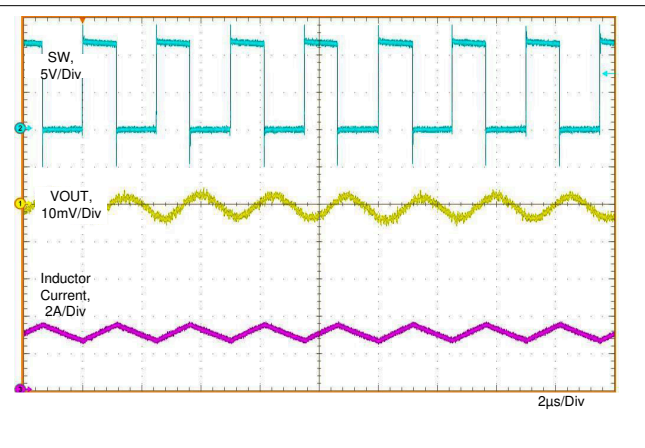
Figure 8-8. Typical PWM Switching Waveforms V_{IN} = 12\text{ V} , V_{OUT} = 5\text{ V} , I_{OUT} = 3\text{ A} , f_S = 400\text{ kHz}
