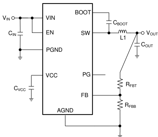
Simplified Schematic
