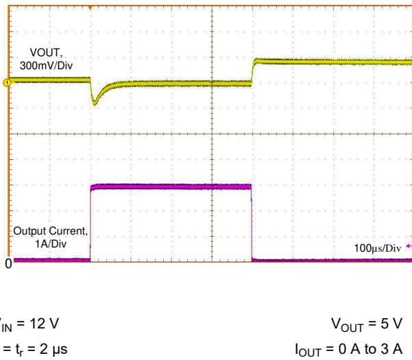
Figure 9-23. Load Transient
