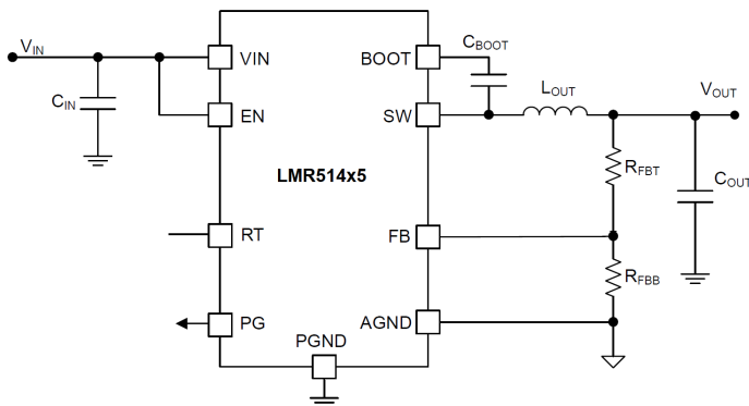
Simplified Schematic
