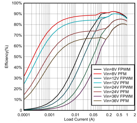
Figure 6-2. 3.3-V Efficiency Versus Load Current
