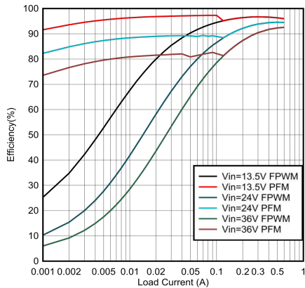
Figure 6-3. 5-V Efficiency Versus Load Current
