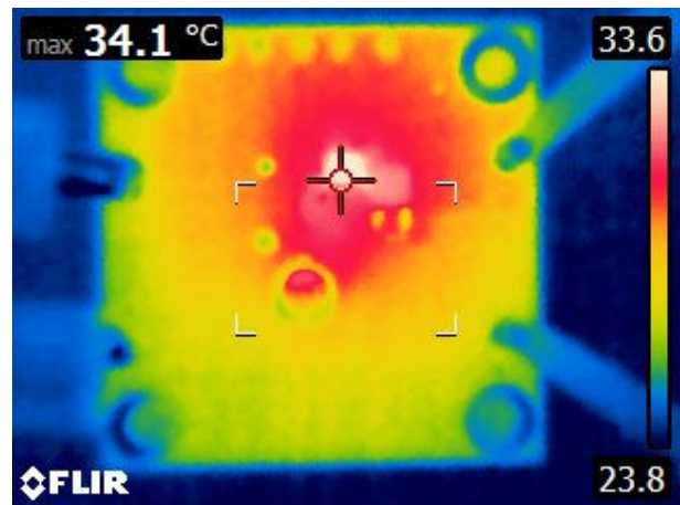
Figure 8-9. Short-Circuit Applied
