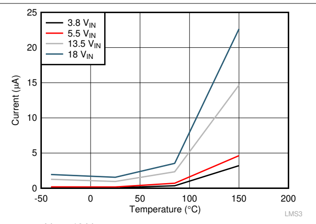
Figure 7-6. Shutdown Current
