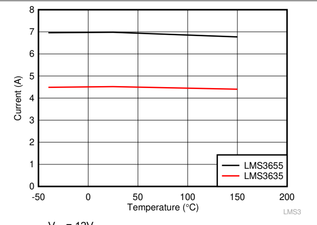
Figure 7-4. Low-Side/Valley Current Limit for LMS36x5-Q1
