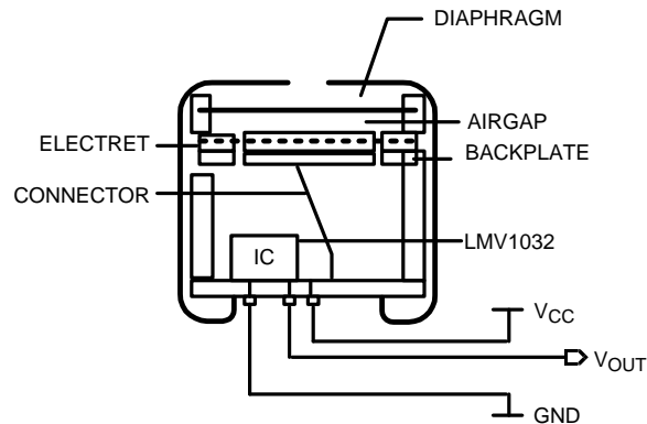
Figure 20. Built-in Gain
