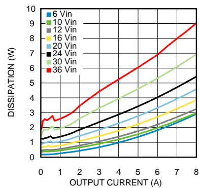
Figure 2. Dissipation 5-V Output at 25°C
