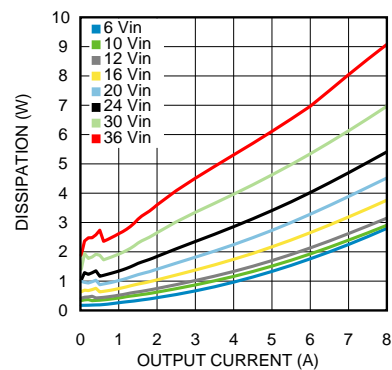
Figure 4. Dissipation 3.3-V Output at 25°C
