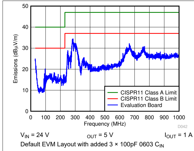
Figure 6-7. Radiated EMI
