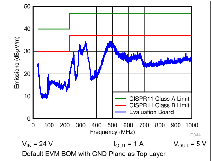
Figure 6-8. Radiated EMI
