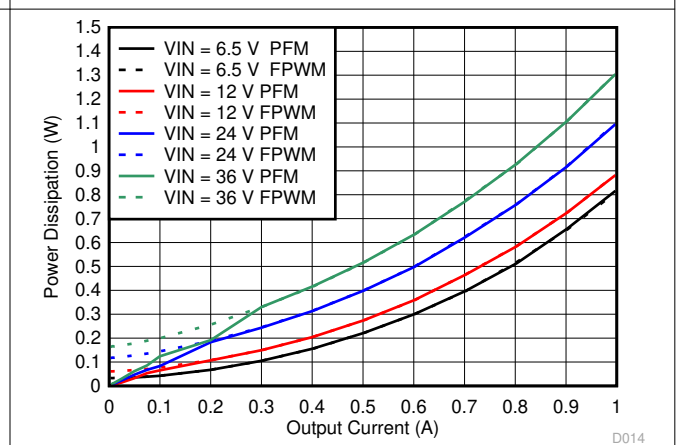
Figure 6-10. Power Dissipation
