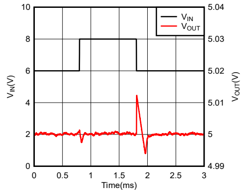
Figure 5-36. Line Transient Response vs Time (New Chip) V_{IN} = 6V to 8V , V_{OUT} = 5V , C_{OUT} = 1\mu F , I_{OUT} = 100\mu A
