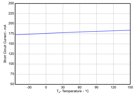
V_{IN} = 6\text{V}, V_{OUT} = 0\text{V} Figure 5-22. Short-Circuit Current vs Temperature (New Chip)
