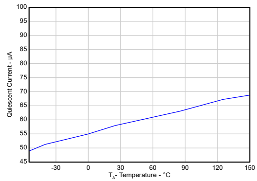
V_{IN} = 6\text{V}, V_{OUT} = 5\text{V} Figure 5-20. Quiescent Current vs Temperature ( I_L = 100\mu\text{A} ) (New Chip)
