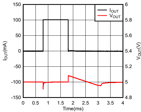
Figure 5-39. Load Transient Response vs Time (New Chip) V_{IN} = 6V , V_{OUT} = 5V , I_{OUT} = 0 to 100mA , C_{OUT} = 1\mu F
