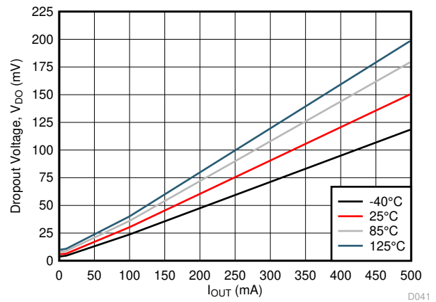
Figure 6-44. LP5912-1.8 Dropout Voltage (V DO ) vs I OUT
