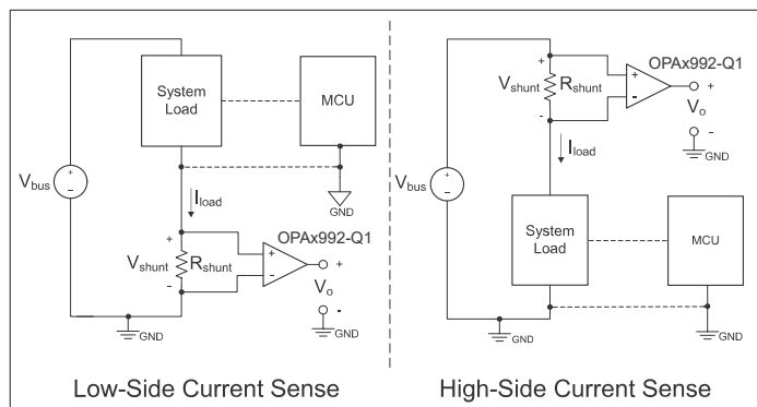
OPAx992-Q1 in Current-Sensing Applications
