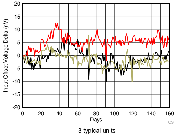
Figure 6-7. Offset Voltage Long Term Drift
