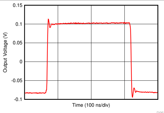
See Figure 8-1, gain = 1 V/V, R_F = 0\ \Omega , C_L = 10\text{ pF}
