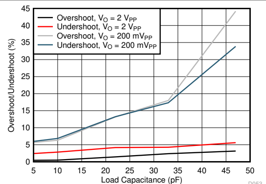
See Figure 8-1, gain = 1 V/V, R_F = 0\ \Omega
