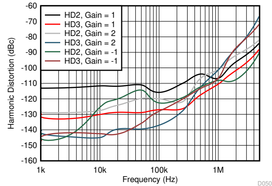
See Figure 8-1 and Figure 8-2, R_F = 0\ \Omega
