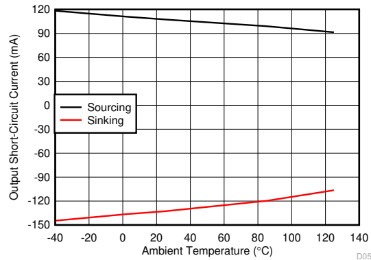
Output saturated and then short-circuited Figure 6-16. Output Short-Circuit Current vs Ambient Temperature
