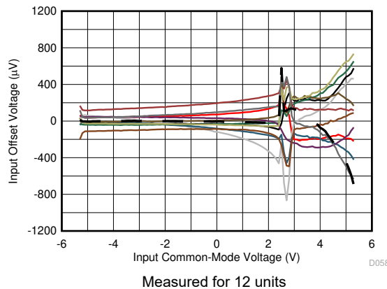
Measured for 12 units Figure 6-17. Input Offset Voltage vs Input Common-Mode Voltage
