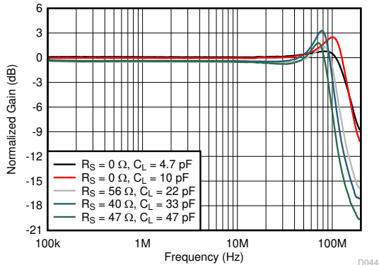
See Figure 8-1 and Figure 7-1, V_O = 20\text{ mV}_{PP} , gain = 1 V/V, R_F = 0\ \Omega
