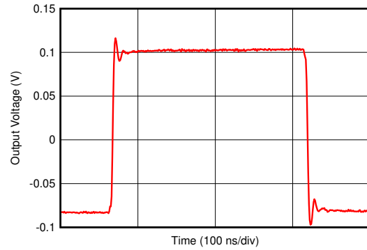
Figure 6-35. Small-Signal Transient Response
