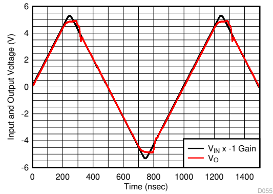
See Figure 8-2, gain = -1 V/V Figure 6-14. Output Overdrive Recovery
