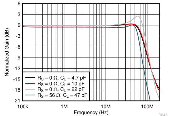
See Figure 8-1 and Figure 7-1, V_O = 20\text{ mV}_{PP} , gain = 2 V/V
