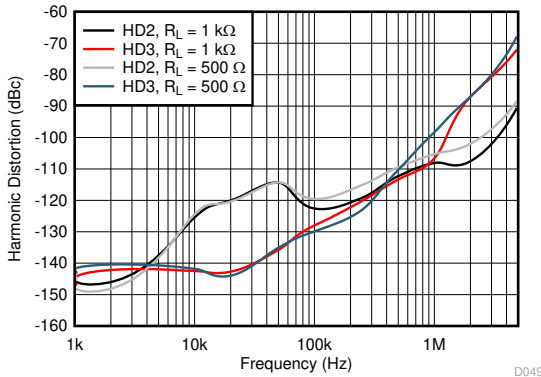
See Figure 8-2, gain = -1 V/V
