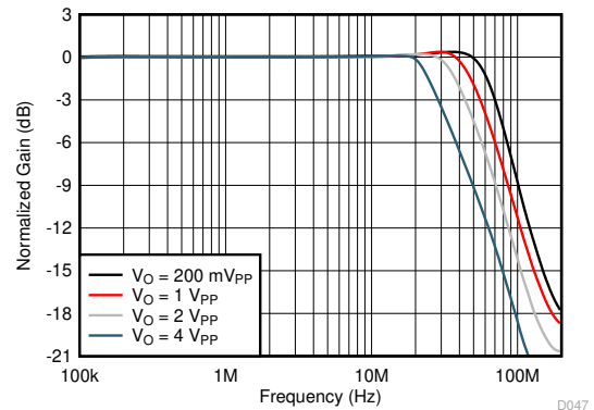
See Figure 8-1, gain = 2 V/V
