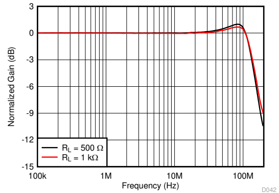
See Figure 8-1, V_O = 20\text{ mV}_{PP} , gain = 1 V/V, R_F = 0\ \Omega
