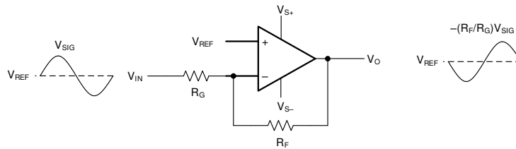
Figure 8-2. Inverting Amplifier
