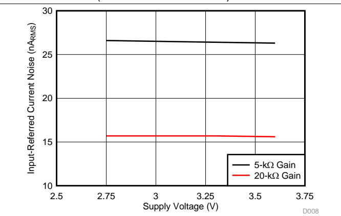
Figure 8. RMS Input-Referred Current Noise vs Supply Voltage
