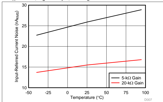
Figure 7. RMS Input-Referred Current Noise vs Temperature
