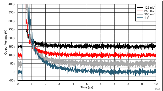
Figure 41. Long-Term Settling Response vs Output Voltage
