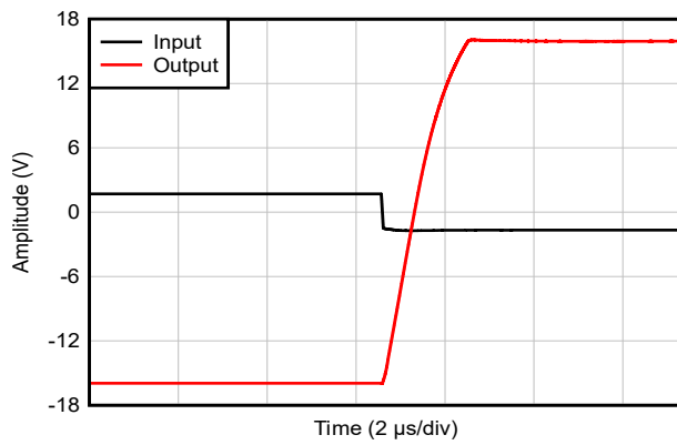
G = -10 Figure 5-43. Negative Overload Recovery
