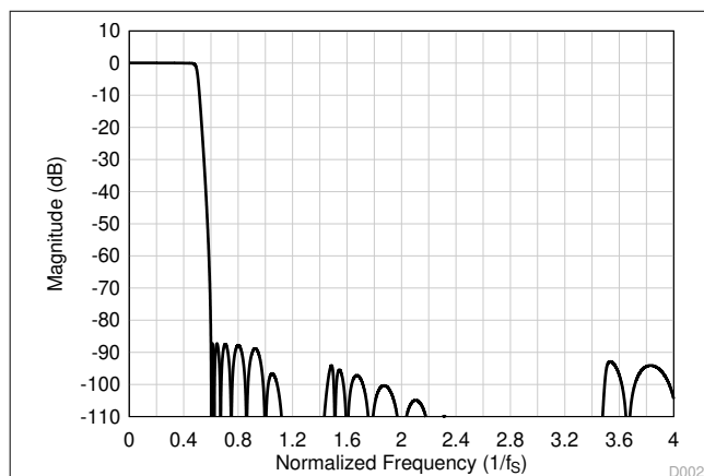
Figure 8-37. Low-Latency Decimation Filter Magnitude Response
