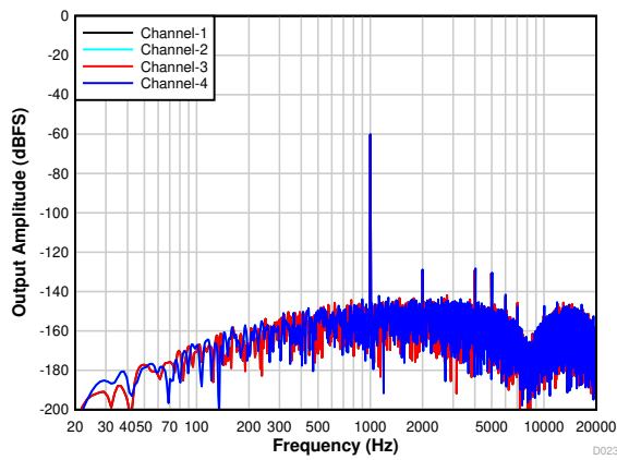
Figure 7-30. PDM Input FFT With a -60-dBr Input
