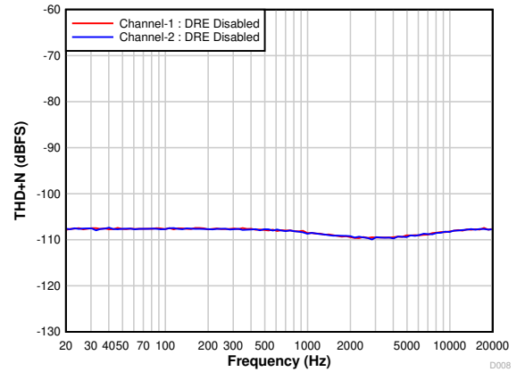
Figure 7-11. THD+N vs Input Frequency With a -60-dBr Input
