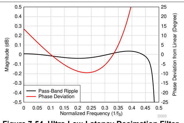
Figure 7-54. Ultra-Low-Latency Decimation Filter Pass-Band Ripple and Phase Deviation
