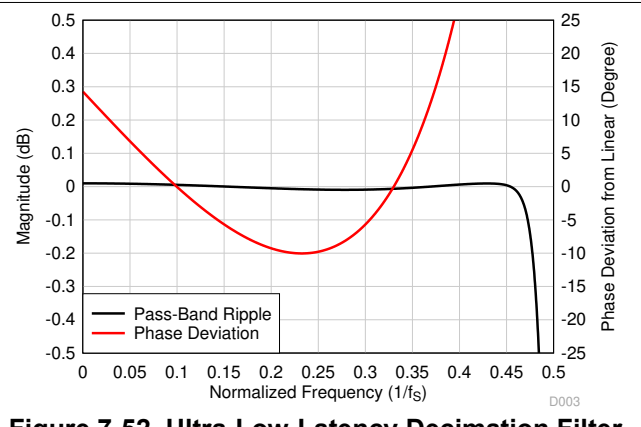
Figure 7-52. Ultra-Low-Latency Decimation Filter Pass-Band Ripple and Phase Deviation
