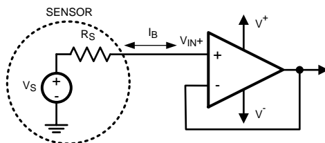
Figure 49. Noise Due to I_{BIAS}
