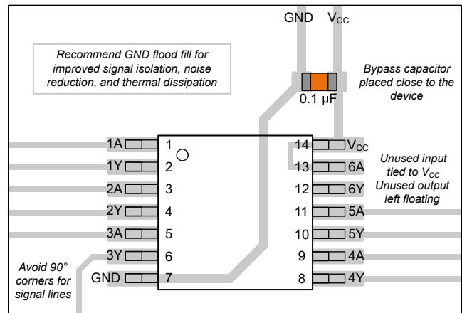
Figure 8-3. Example Layout for the SN54SC6T07-SEP
