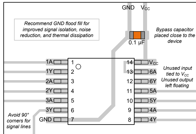
Figure 8-3. Example Layout for the SN54SC6T14-SEP
