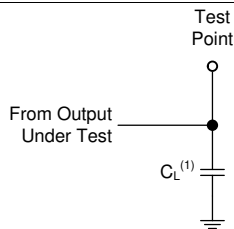
C_L = 50 pF and includes probe and jig capacitance. Figure 5. Load Circuit
