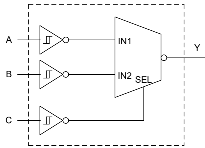
2 to 1 Data Selector with inverted output Y = A when C is H Y = B when C is L
