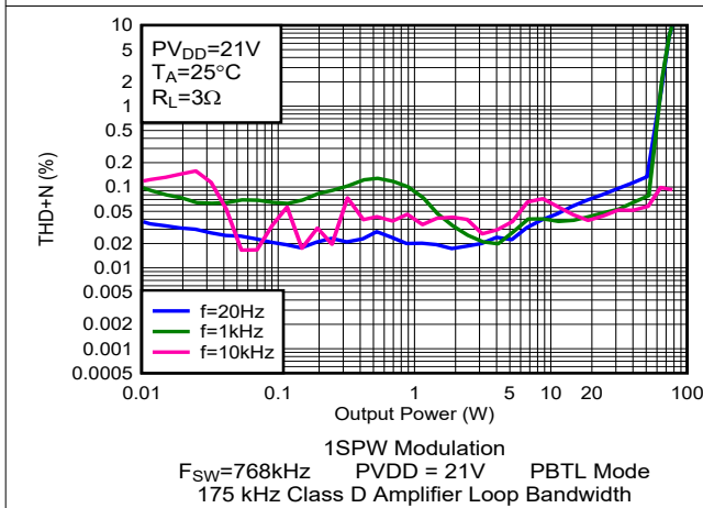
Figure 6-104. THD+N vs Output Power
