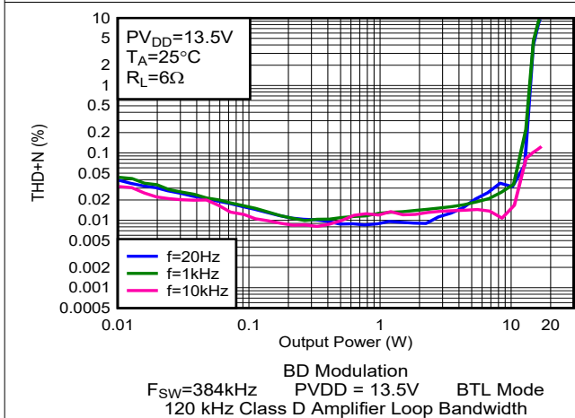
Figure 6-19. THD+N vs Output Power
