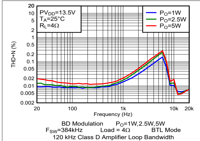
Figure 6-1. THD+N vs Frequency
