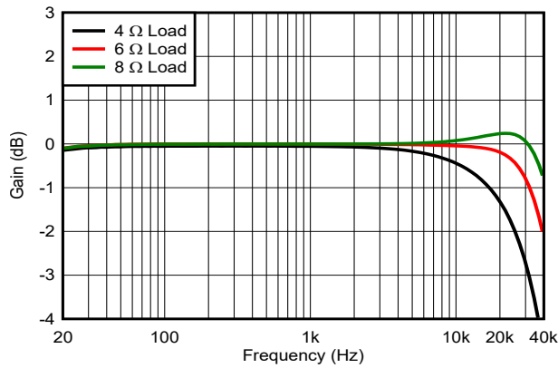
BD Modulation P_O=1W PVDD=21V F sw =384kHz BTL Mode 120 kHz Class D Amplifier Loop Bandwidth
