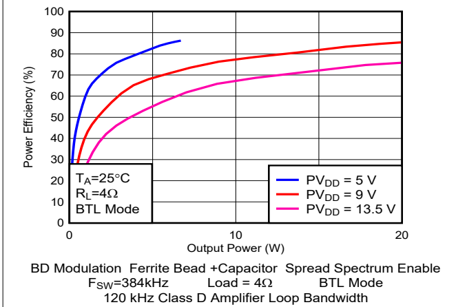
Figure 6-43. Efficiency vs Output Power (with FB)
