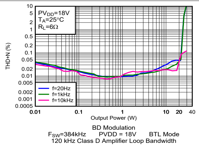
Figure 6-20. THD+N vs Output Power
