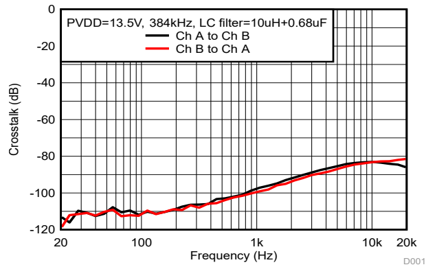
PVDD=13.5V BD Modulation Pout=1W F sw =384kHz Load = 6Ω BTL Mode
