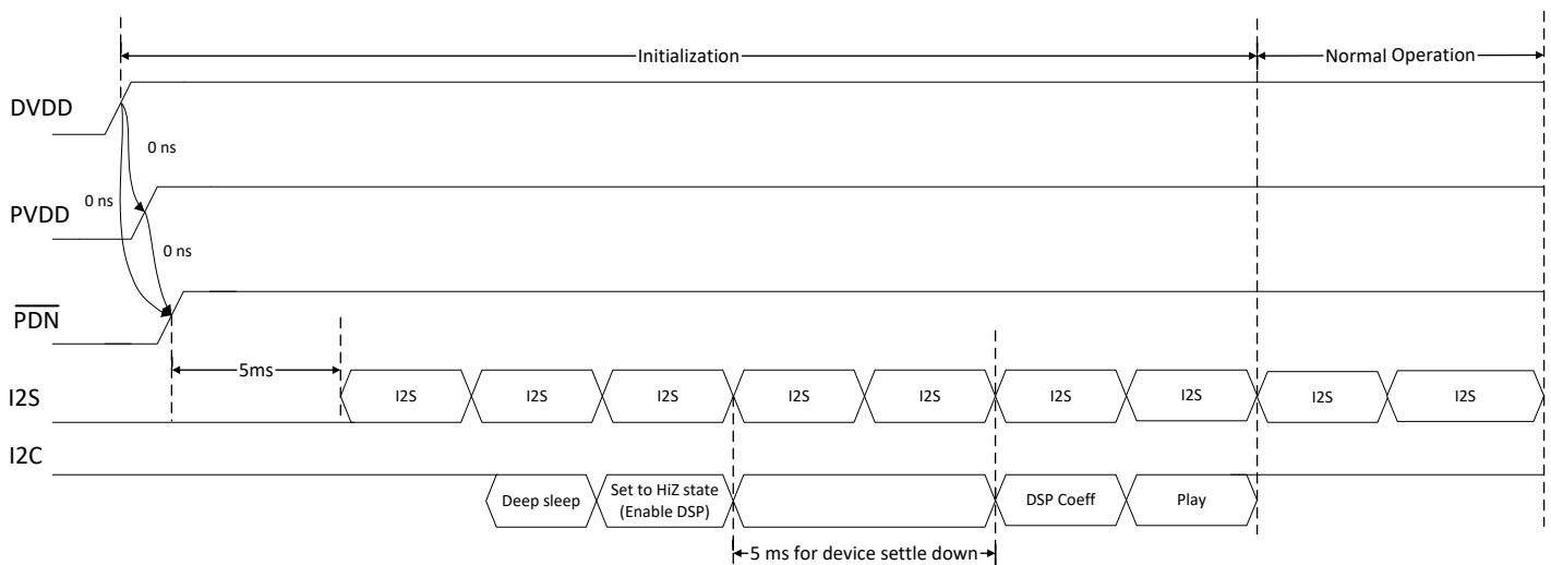
Figure 7-14. Startup sequence
