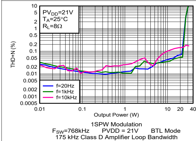
Figure 6-68. THD+N vs Output Power
