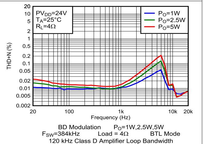
Figure 6-4. THD+N vs Frequency
