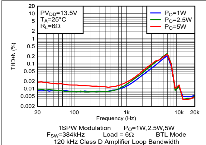
Figure 6-5. THD+N vs Frequency
