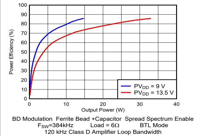
Figure 6-44. Efficiency vs Output Power
