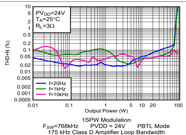
Figure 6-105. THD+N vs Output Power
