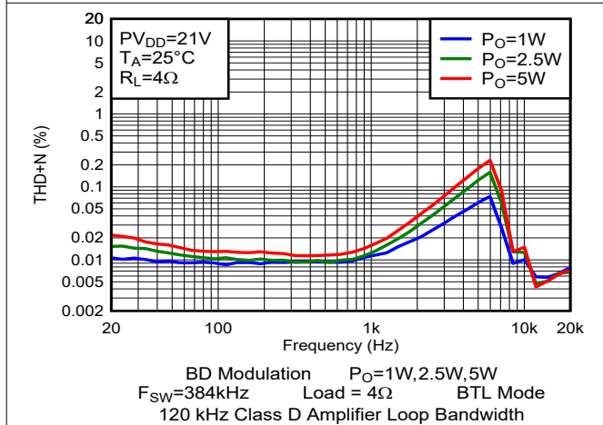
Figure 6-3. THD+N vs Frequency
