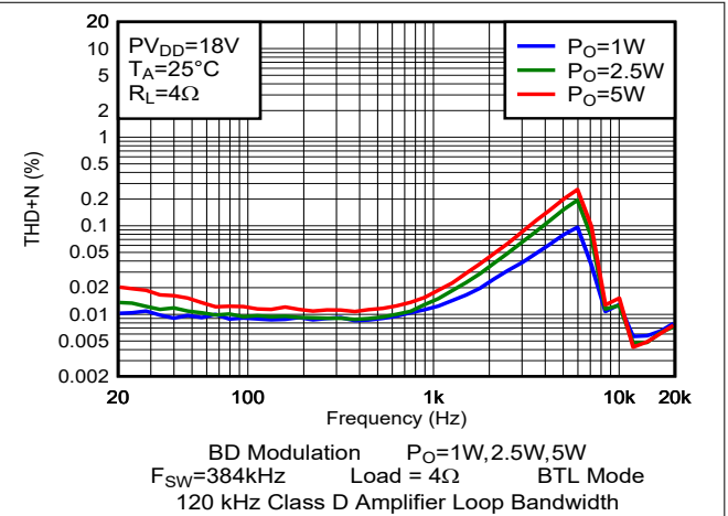
Figure 6-2. THD+N vs Frequency
