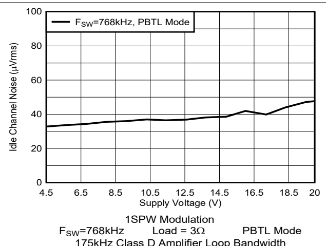
Figure 6-107. Idle Channel Noise vs Supply Voltage
