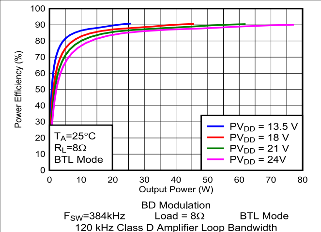
Figure 6-42. Efficiency vs Output Power
