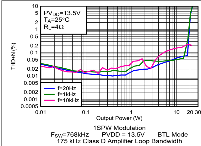
Figure 6-58. THD+N vs Output Power
