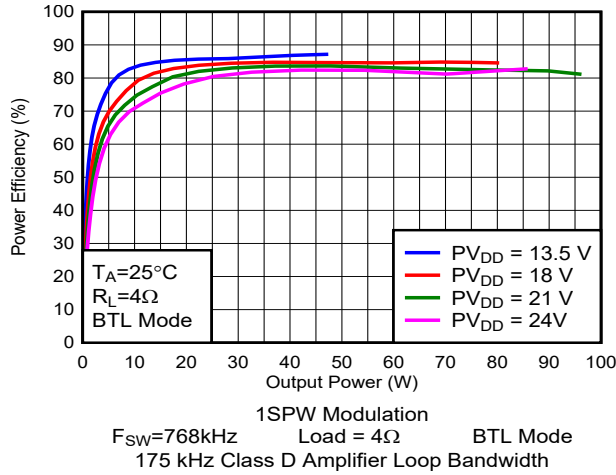
Figure 6-82. Efficiency vs Output Power
