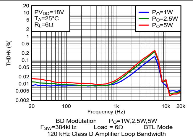
Figure 6-6. THD+N vs Frequency
