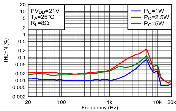
Figure 6-54. THD+N vs Frequency
