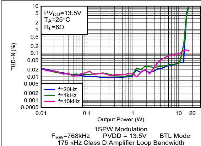
Figure 6-62. THD+N vs Output Power
