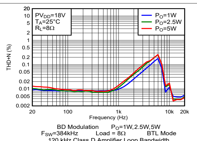
Figure 6-10. THD+N vs Frequency
