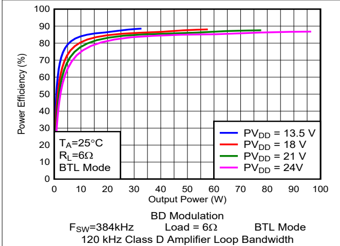
Figure 6-41. Efficiency vs Output Power
