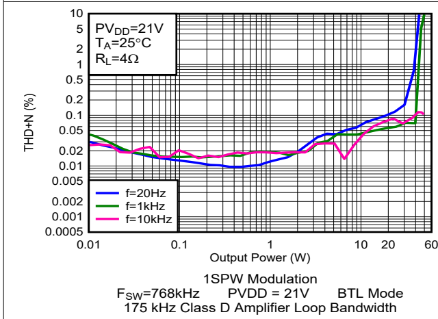
Figure 6-60. THD+N vs Output Power
