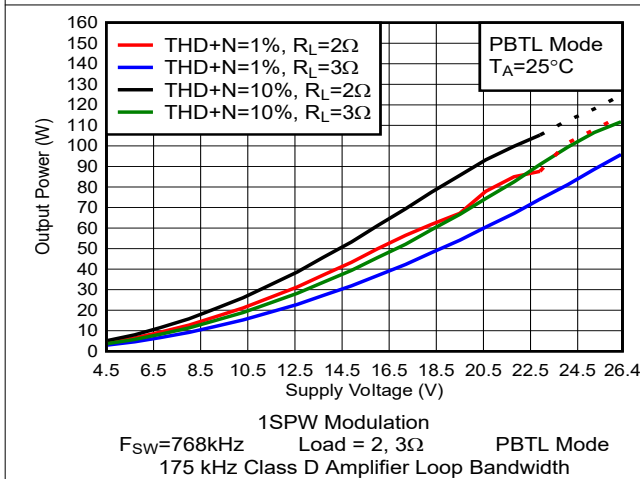
Figure 6-106. Output Power vs Supply Voltage (dotted line is thermally limited)
