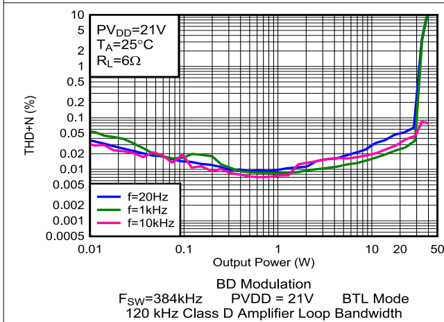
Figure 6-21. THD+N vs Output Power
