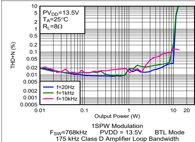
Figure 6-66. THD+N vs Output Power
