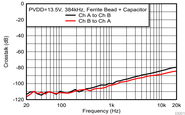
Spread Spectrum Enable BD Modulation Load = 6Ω Pout=1W BTL Mode
