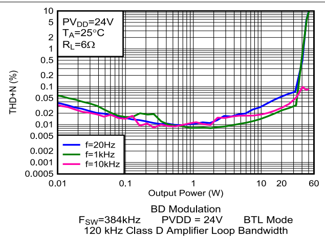
Figure 6-22. THD+N vs Output Power
