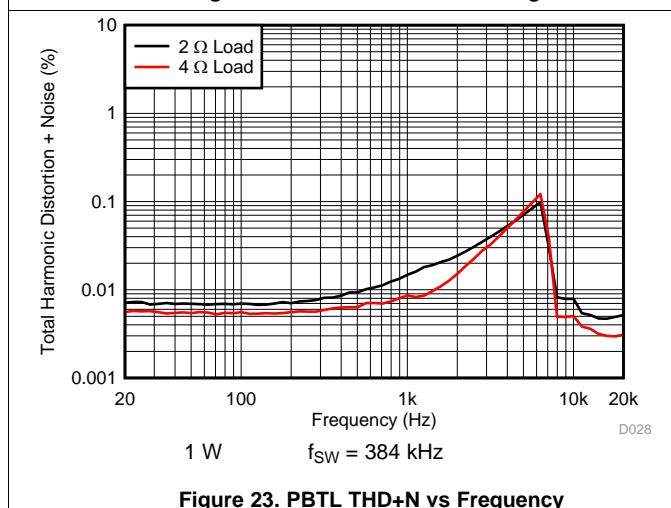
Figure 23. PBTL THD+N vs Frequency
