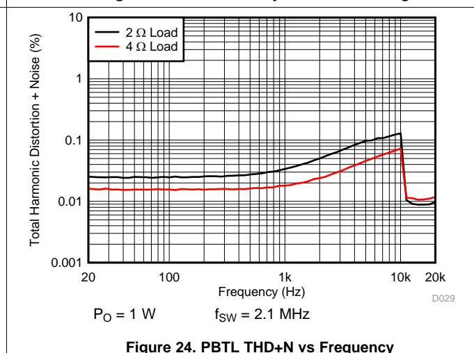
Figure 24. PBTL THD+N vs Frequency
