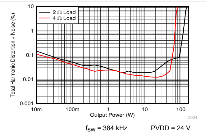
Figure 7-28. PBTL THD+N vs Power
