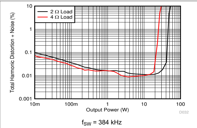
Figure 7-26. PBTL THD+N vs Power
