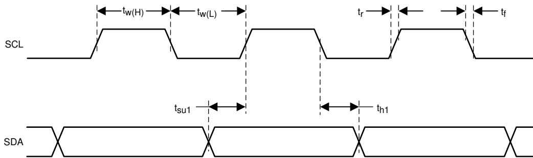
Figure 9-10. SCL and SDA Timing
