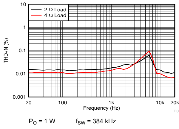
Figure 7-22. PBTL THD+N vs Frequency
