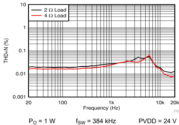
Figure 7-24. PBTL THD+N vs Frequency
