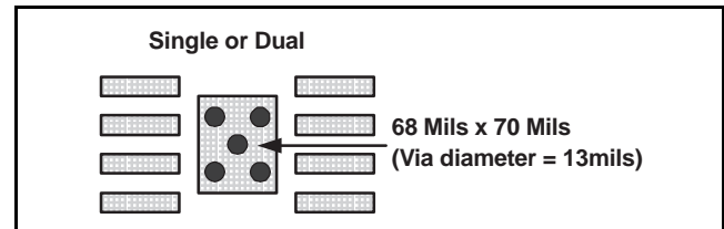
Figure 90. PowerPAD PCB Etch and Via Pattern
