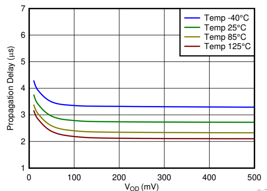
Propagation Delay vs. Input Overdrive
