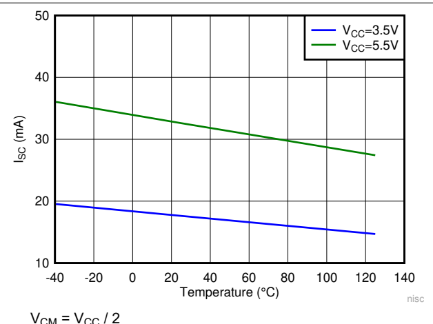
Figure 6-18. Output Short-Circuit (Sink) Current vs Temperature
