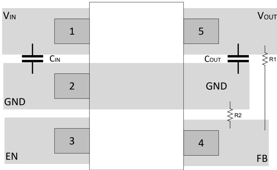
Figure 7-2. DBV Package (SOT-23) Typical Layout
